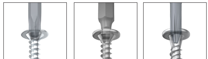
#2 Mod. Phillips Combo Driver #2 Square Drive System #2 Phillips Drive System
